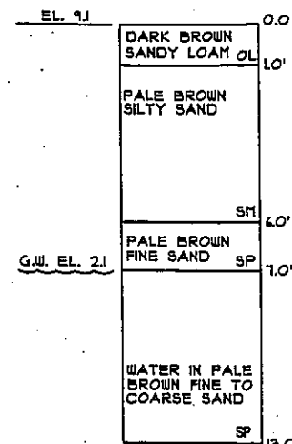
TEST HOLE BY McDONALD GEOSCIENCE 01.02.01 NO SCALE
