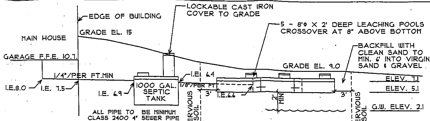
PROFILE @ GARAGE NO SCALE
